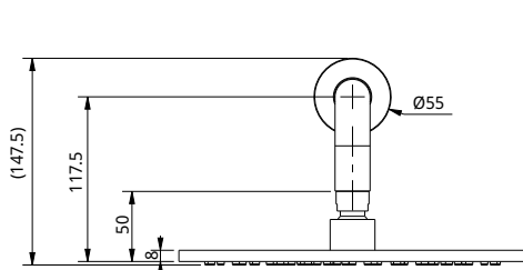
Dimensions shown with the 250mm overhead shower
