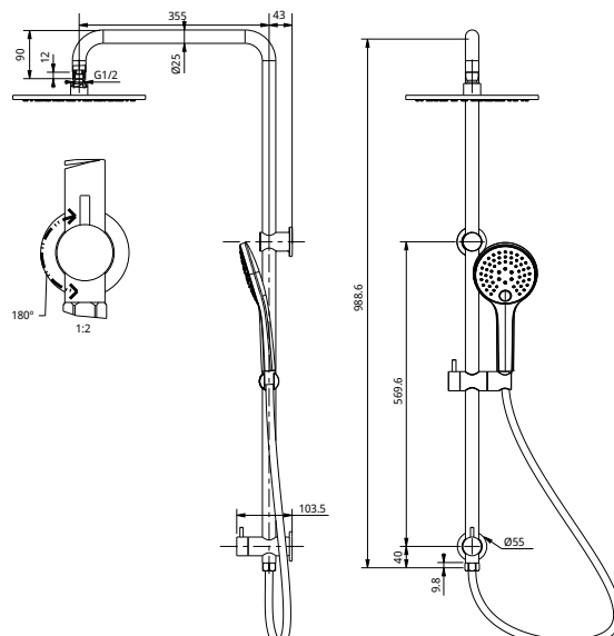
Bottom inlet
