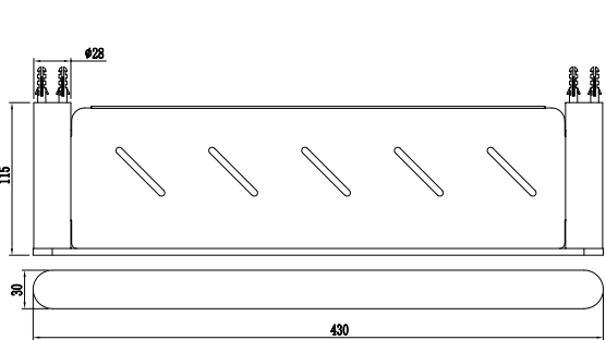
WSPAPSSCP/BN/GM WSELSS430MB
