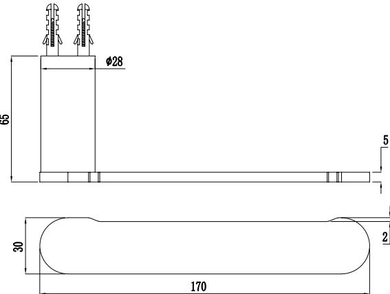
WSPAPHT220CP/BN/GM WSELTBMB/WSPAPTBM
